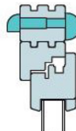
Installation in attachment profile
